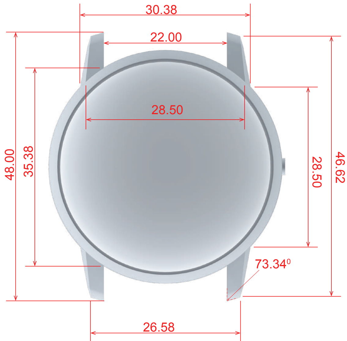
WATCH CASE
